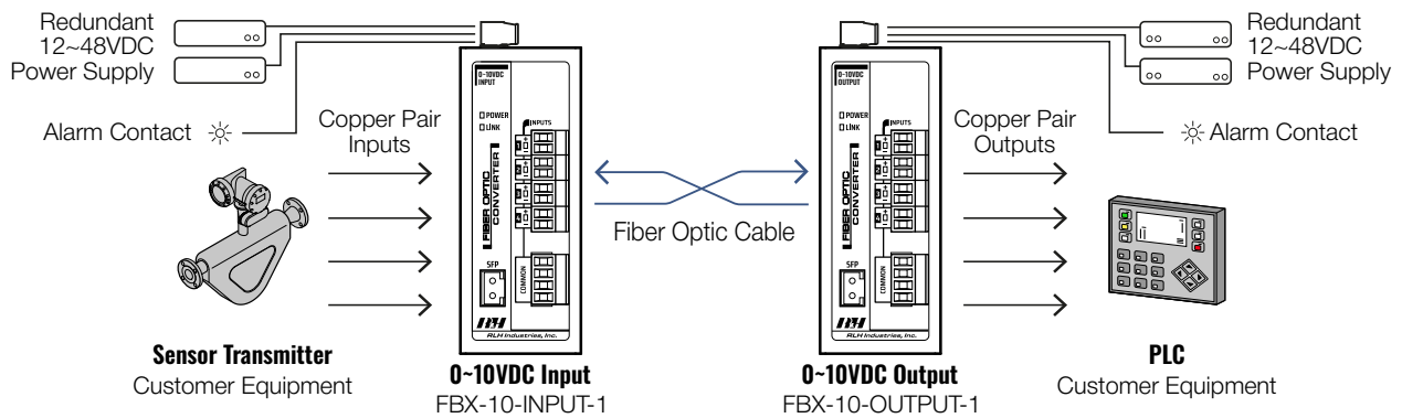
System Diagram
