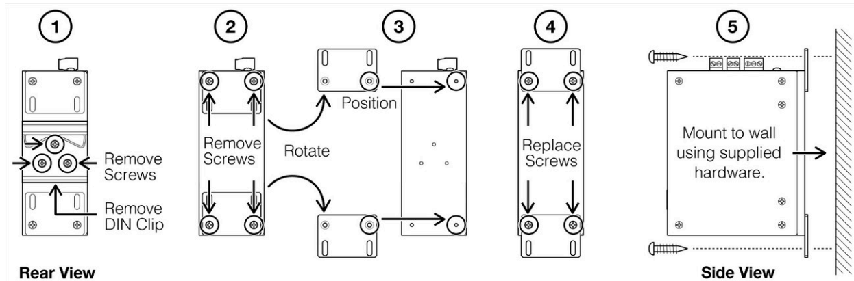
Wall Mounting
